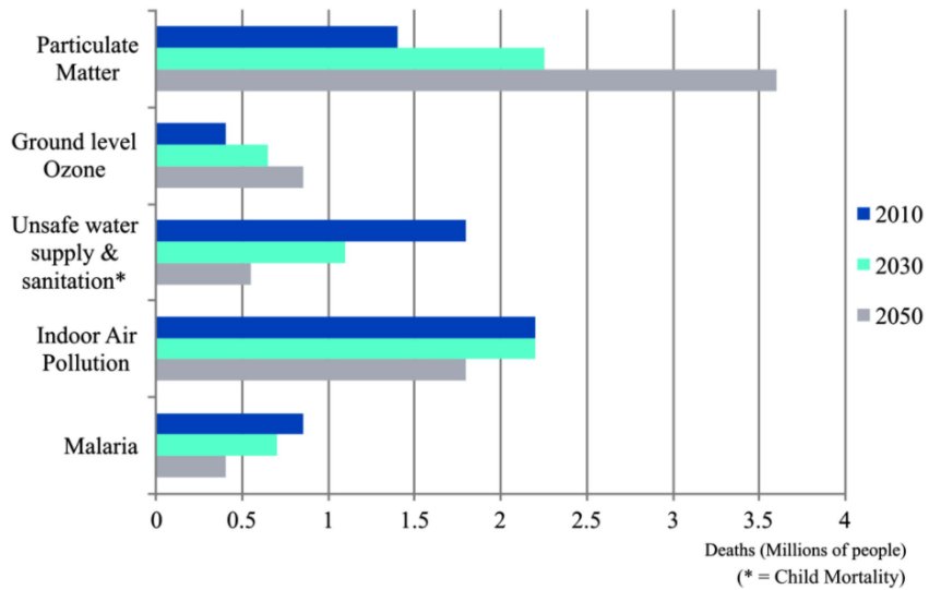
Global premature deaths from selected environmental risks: Baseline, 2010 to 2050
